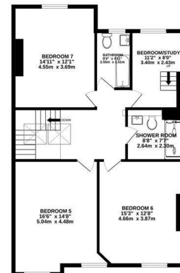
2ND FLOOR - ROOM HEIGHT = 2.75M
